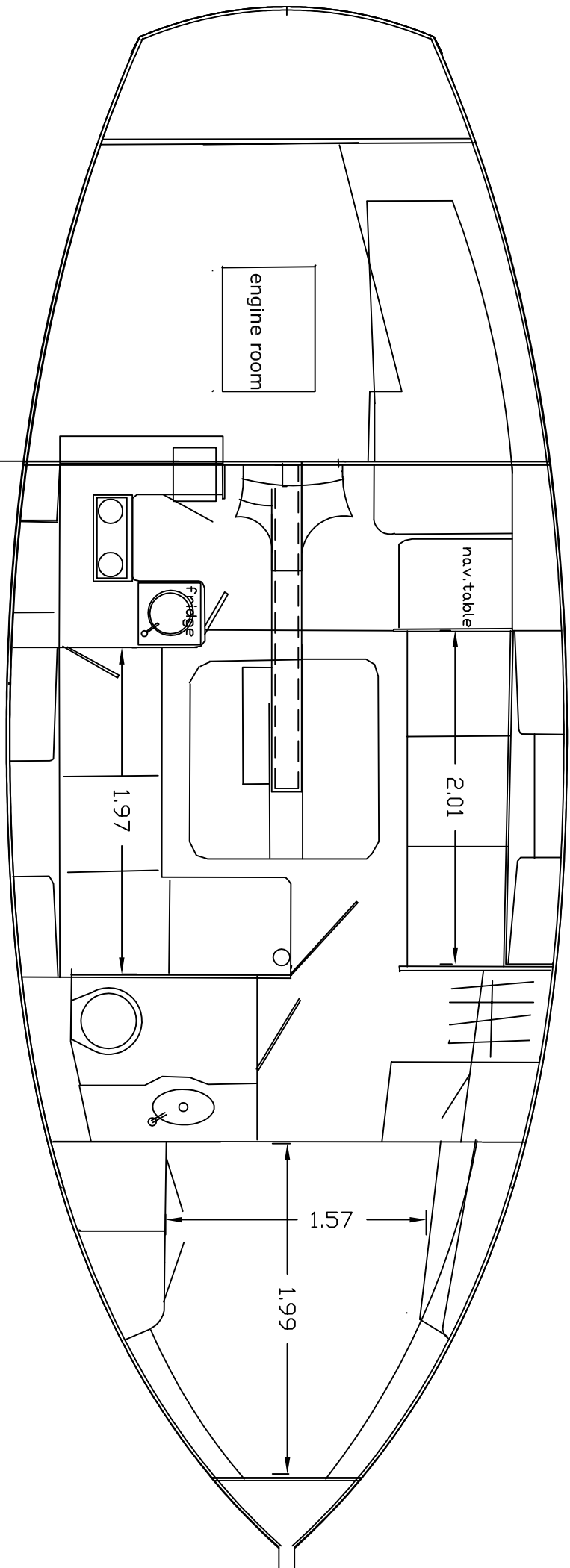
interior with navigation table and 1 pilot berth
